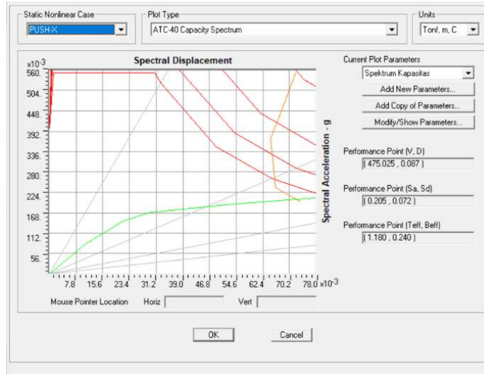
Gambar 4. Performance Point Arah x
