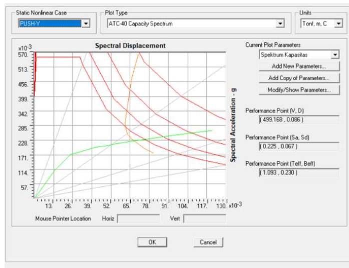
Gambar 5. Performance Point Arah y
